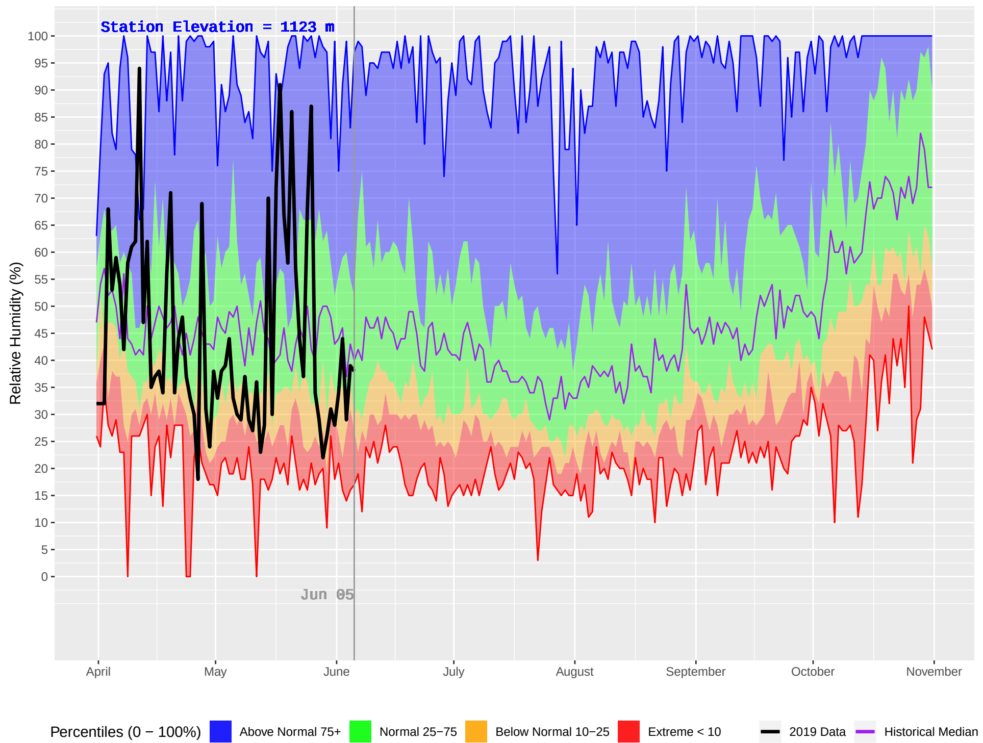
MCLEAN LAKE (311) : Historical (1987–2018) and Current (2019) Daily Relative Humidity
