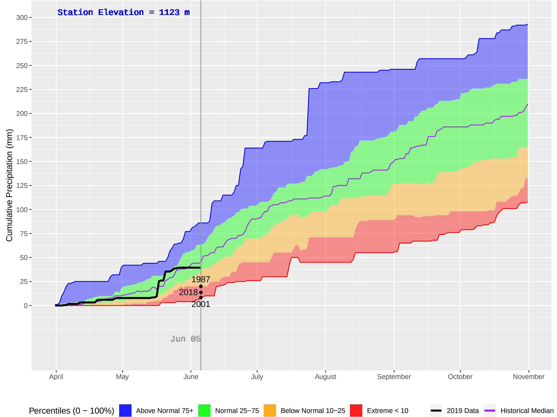
MCLEAN LAKE (311) : Historical (1987–2018), Current (2019) Daily Cumulative Precipitation
