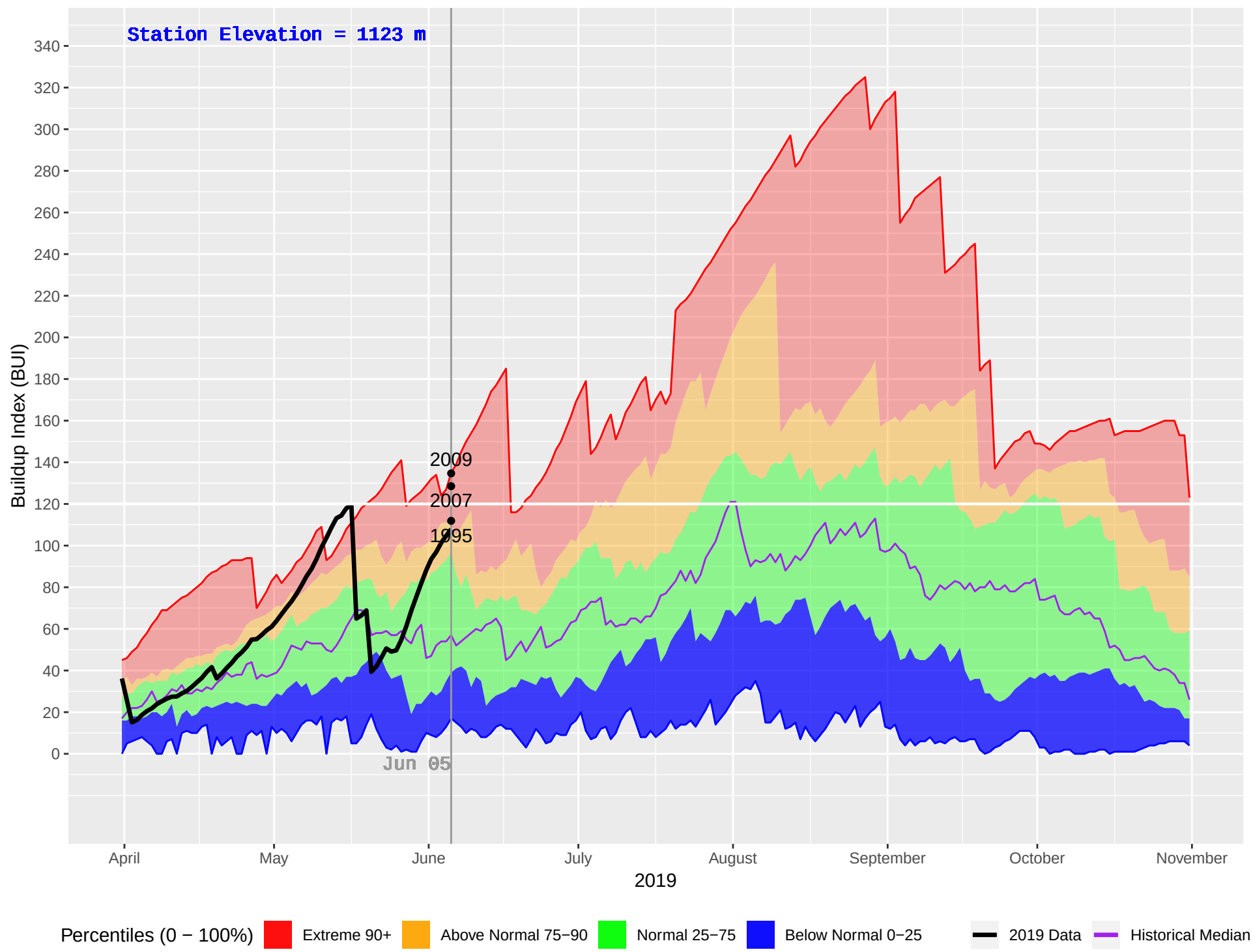
MCLEAN LAKE (311) : Historical (1987–2018), Current (2019) Daily Buildup Index (BUI)
