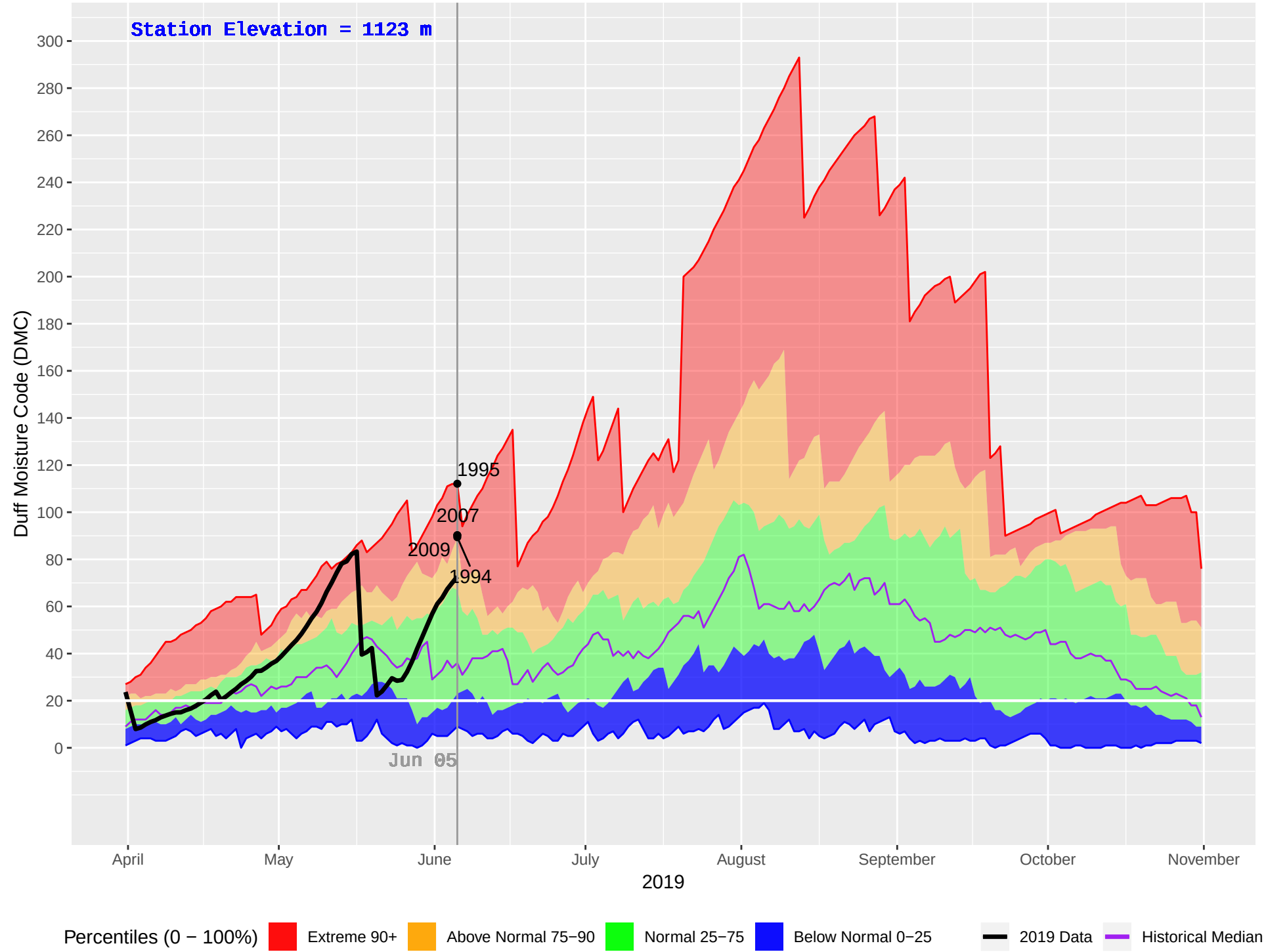
MCLEAN LAKE (311) : Historical (1987–2018), Current (2019) Daily Duff Moisture Code (DMC)
