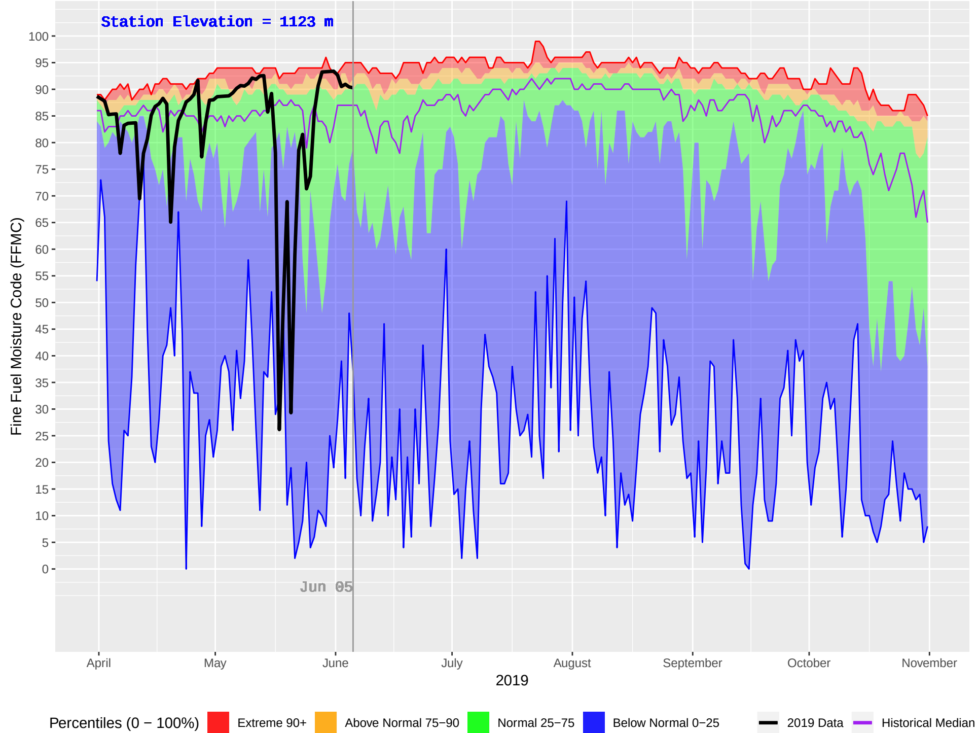
MCLEAN LAKE (311) : Historical (1987–2018) and Current (2019) Daily Fine Fuel Moisture Code (FFMC)
