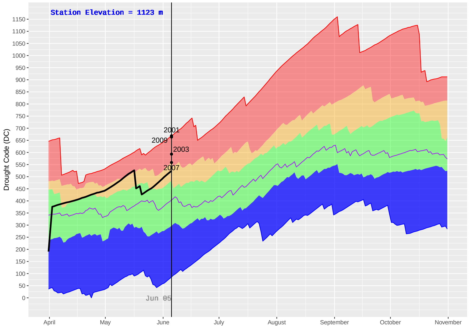
MCLEAN LAKE (311) : Historical (1987–2018) and Current (2019) Daily Drought Code (DC)
