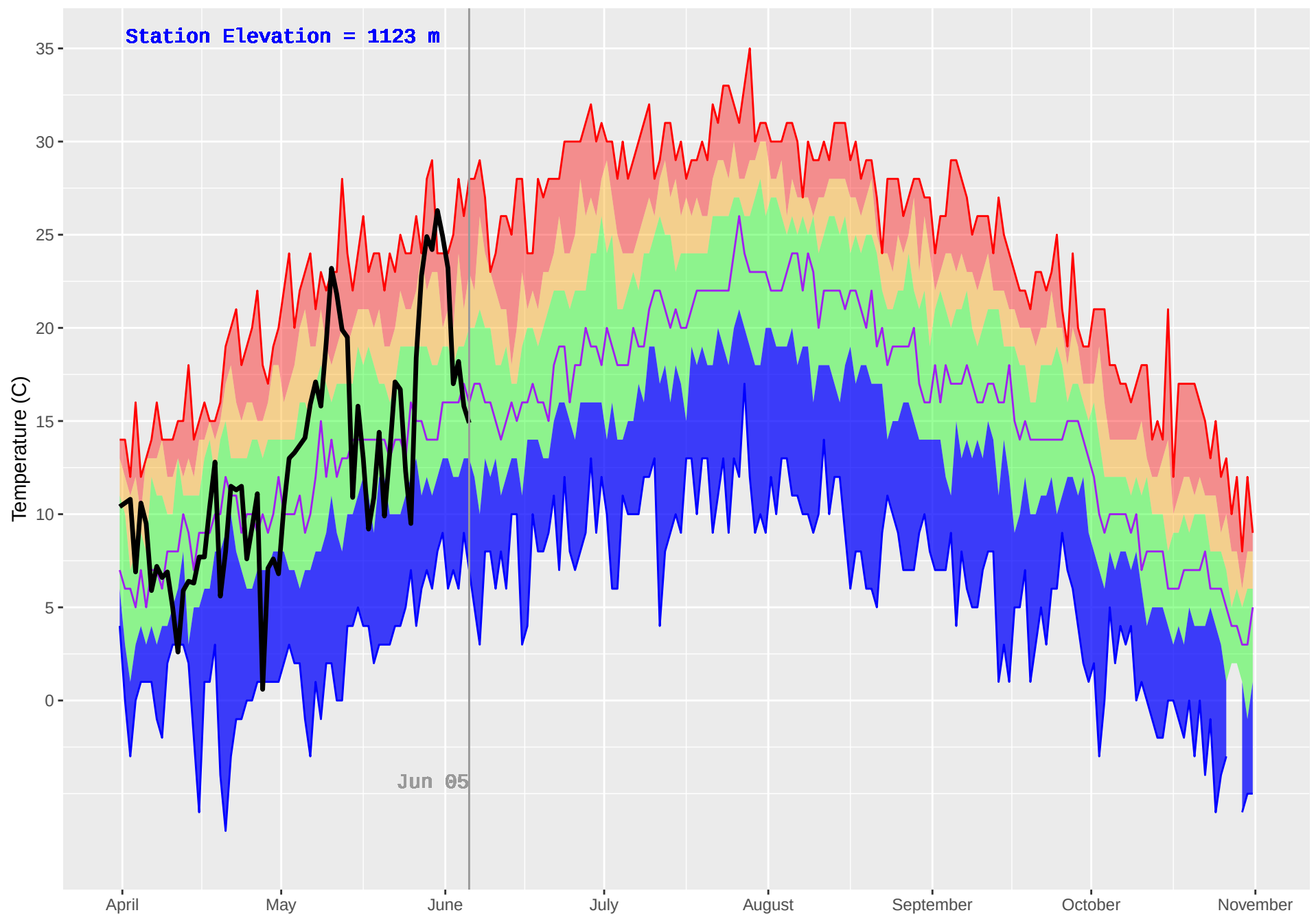
MCLEAN LAKE (311) : Historical (1987–2018) and Current (2019) Daily Temperature
